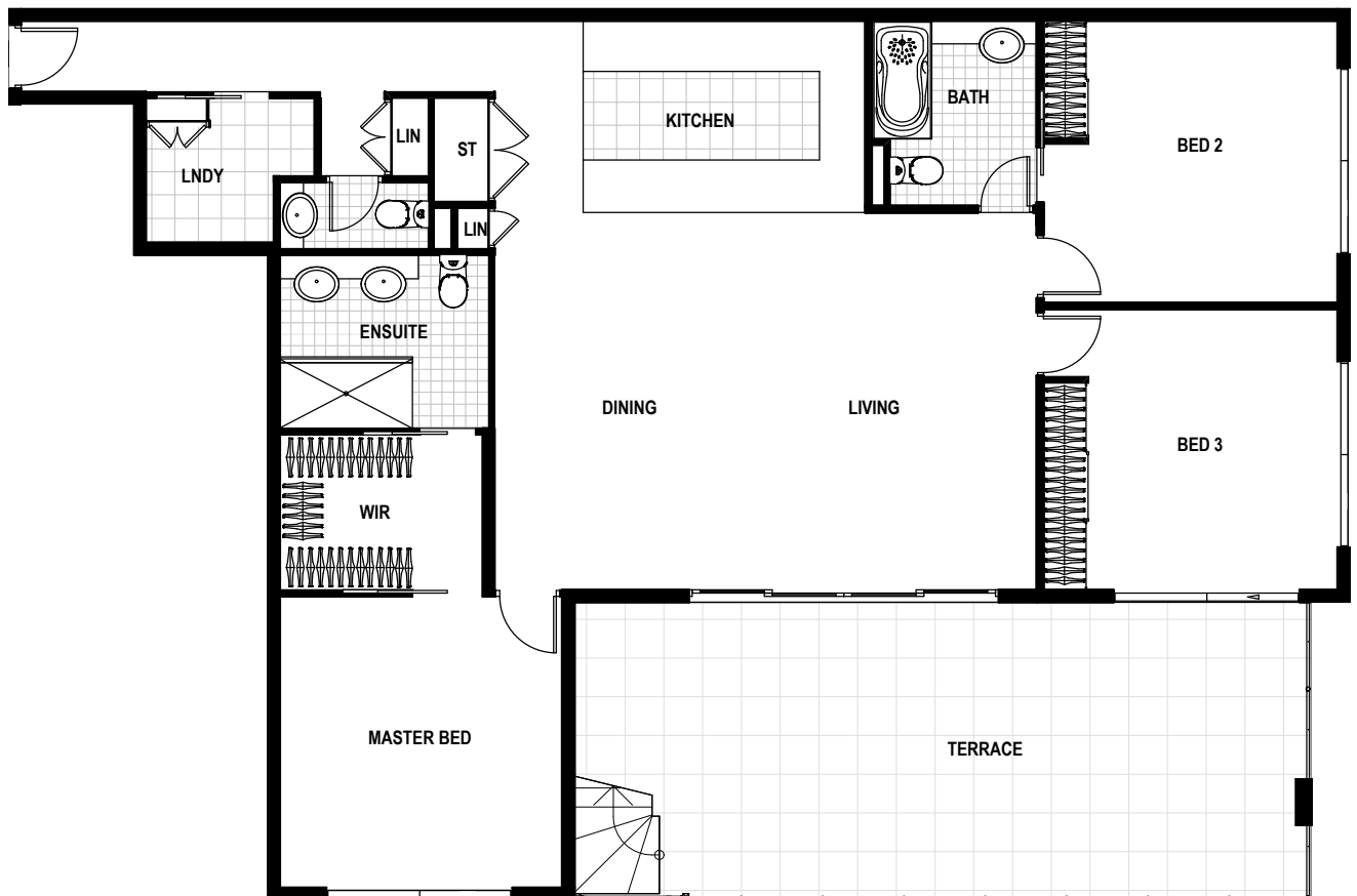
TYPICAL 3 BEDROOM 3 BATHROOM PENTHOUSE FLOOR PLAN 1:100
